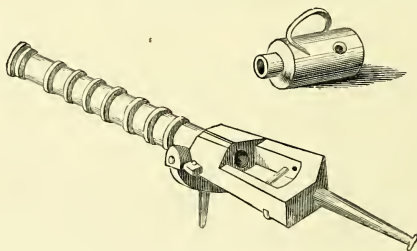
Early English Breech-loading Cannon.
